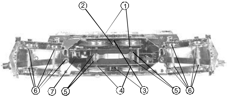
Figure 2: Lubricating Engine
