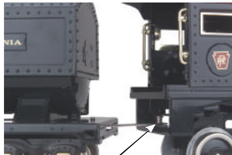
Figure 5: Drawbar Connection
