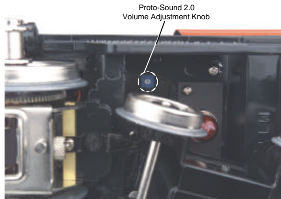
Figure 6: Proto-Sound Manual Volume Adjustment
