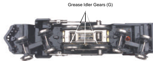
Figure 9 : Greasing the Idler Gears
