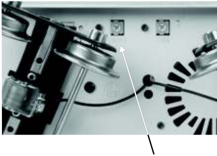
Figure 2: Smoke Unit Control Smoke Unit Control (on bottom of tender)
