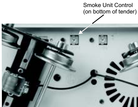
Figure 10: Smoke Unit Control
