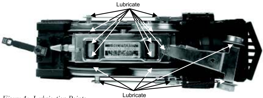
Figure 1: Lubrication Points
