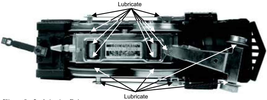
Figure 9: Lubrication Points
