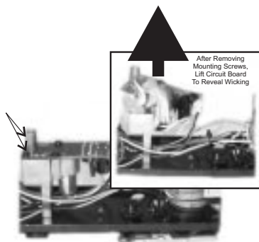
Figure 2: Inspecting The Smoke Unit Wicking
