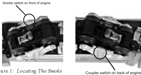
Figure 1: Locating The Smoke Unit & ProtoCoupler Slection
