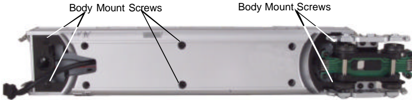
Figure 13a. Locations of Body Mounting Screws.
