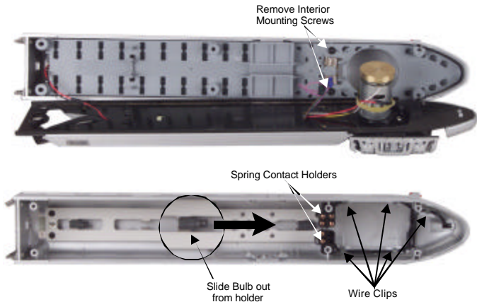
Figure 14c. Locations of the Observation Car screws and the Bulb locations.
