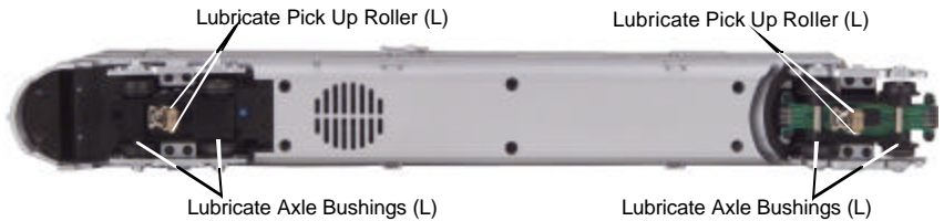
Figure 8. Lubrication Points on the Locomotive
