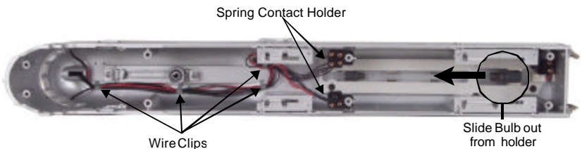
Figure 12b. Replacing the Bulbs inside the shell of the engine.
