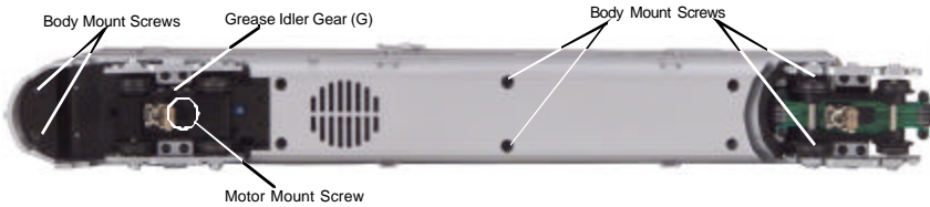
Figure 9. Location of Body Mount Screws and Greasing Points on the Locomotive
