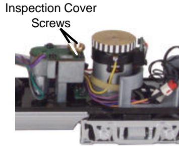
Figure 6. Inspecting the Smoke Unit
