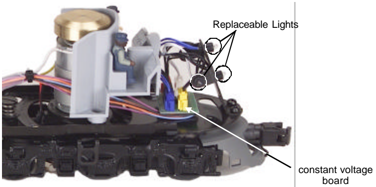
Figure 12a. Locations of Replaceable Lights
