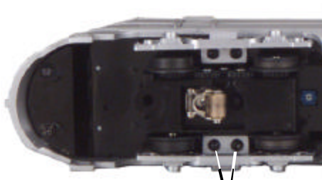
Screws to Remove Trucksides
