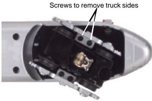
Figure 10b. Changing the traction tires on the rear truck
