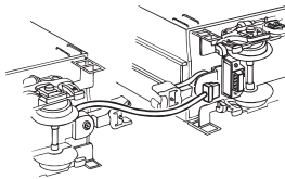
Figure 1: Plugging In the ProtoSound® Cable Harness
