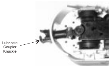
Figure 3: Lubricating The ProtoCoupler Knuckle
