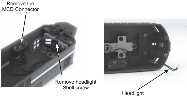
Figure 6. Removing the Headlight
