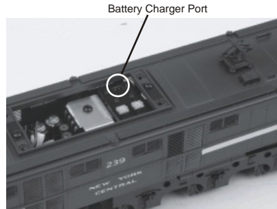
Figure 6. Battery Charger Port location.
