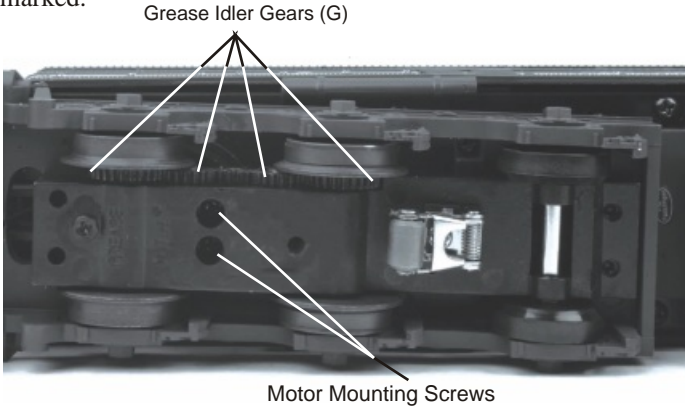
Figure 4. Greasing The Idler Gears
