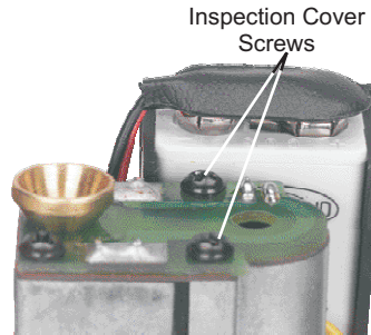
Figure 5. Inspecting the Smoke Unit
