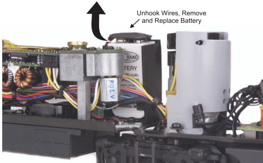
Figure 11. Replacing the Battery and the Location of the Battery Re-charging Jack.
