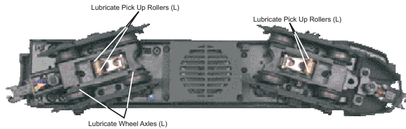
Figure 7. Lubrication Points on the Locomotive
