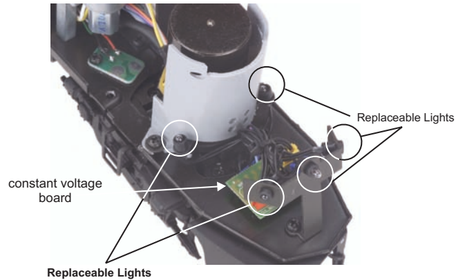
Figure 10. Locations of Replacable Lights
