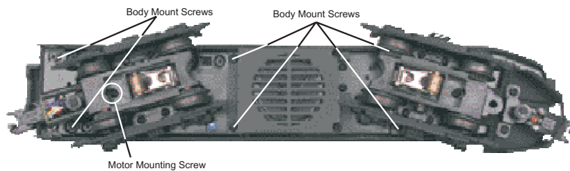
Figure 8. Location of Body Mount Screws and Greasing Points on the Locomotive
