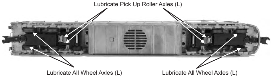
Figure: Lubrication Points
