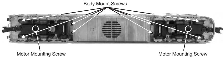
Figure: Body Removal Screw Locations and Motor Mounting Screws
