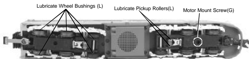
Figure 7: Lubricate The Engine Chassis Trucks
