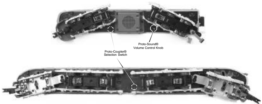
Figure 4: Adjusting The Proto-Sound® Volume and selecting the ProtoCoupler direction.
