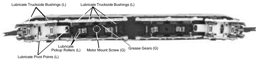
Figure 6: Lubricating The B-Unit Chassis
