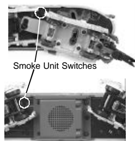
Figure 1: Locating the Smoke Unit Switches on the A and B units
