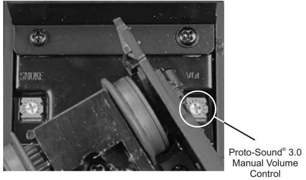
Figure 8: Manual Volume Control
