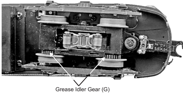
Figure 11: Greasing the Idler Gears
