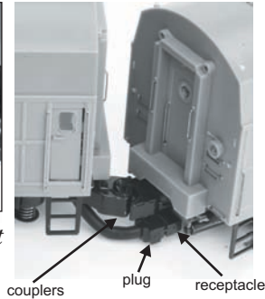
Figure 6: Correct way to Connect wire harness plug into the receptacle
