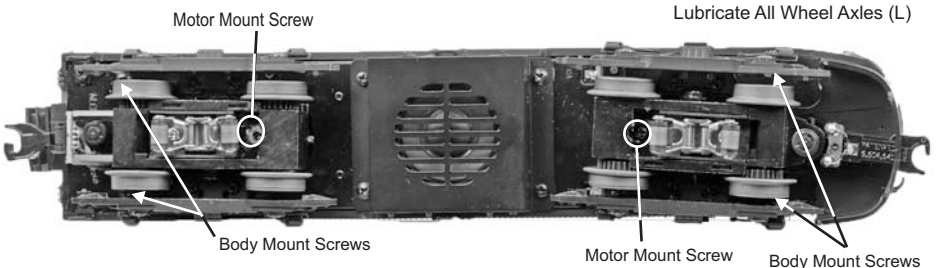
Figure 10: Body Mount Screws
