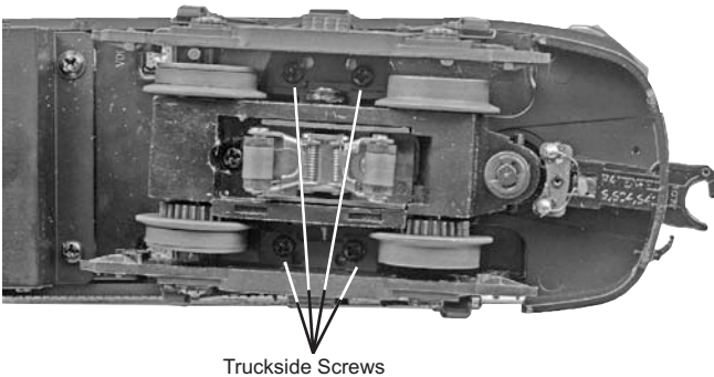
Figure 12: Truckside Screws
