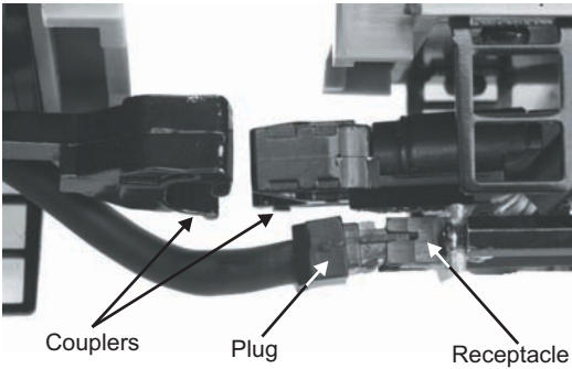
Figure 5: Connecting ABA Units
