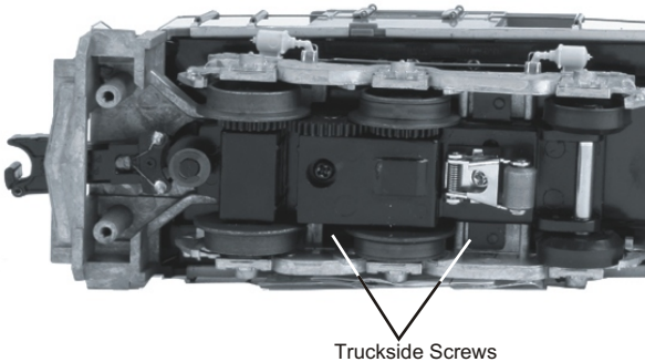
Truckside Screws
