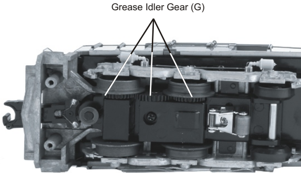
Greasing The Idler Gears
