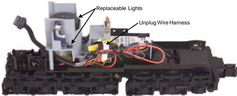
Figure 9. Replacing the Lights in your Engine
