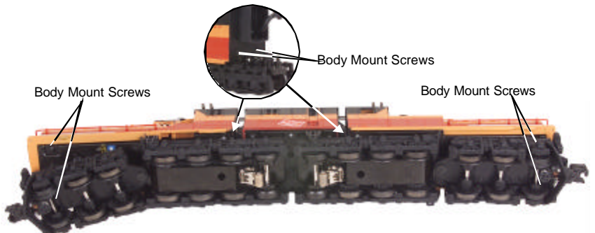
Figure 6. Locations of the Body Mounting Screws
