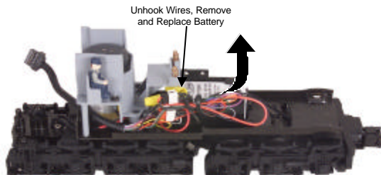
Figure 11. Replacing the Battery
