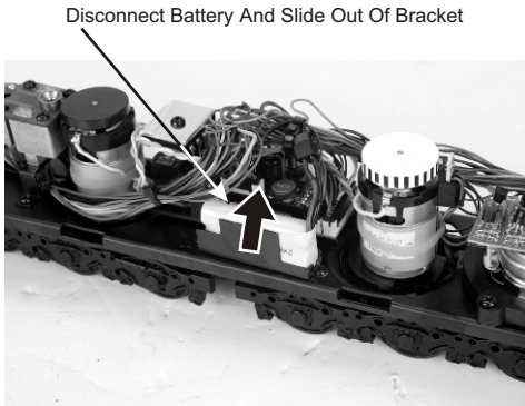
Figure 10. Battery Location.
