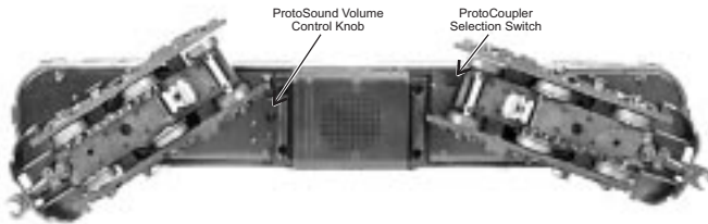
Figure 2: Locating The Proto-Coupler® Selection Switch
