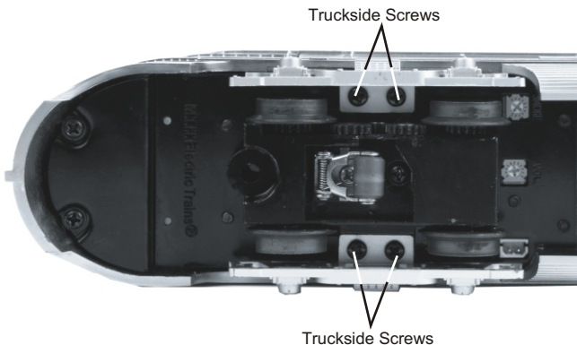
Truckside Screws
