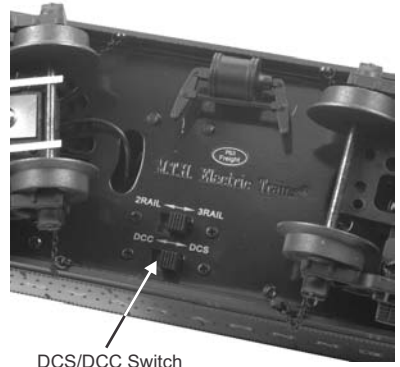
Figure: Changing from DCS to DCC Mode
