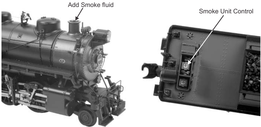
Figure: Adding Smoke Fluid
