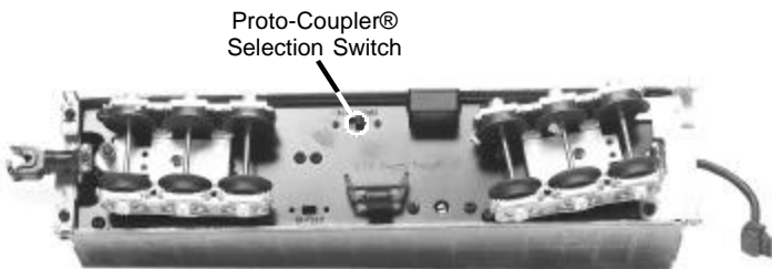
Figure 6b. Selecting the coal tender or Auxiliary tender ProtoCoupler
