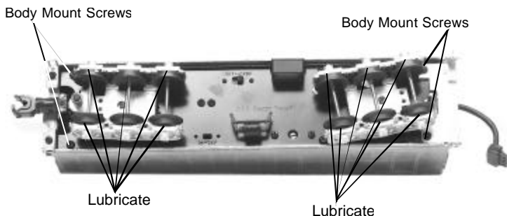
Figure 8: Lubricate The Tender Chassis Trucks
