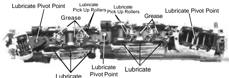
Figure 7: Lubricating The Locomotive Chassis
