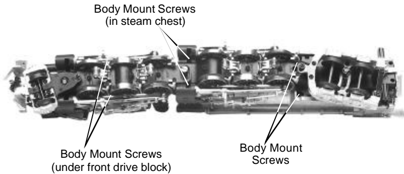
Figure 9: Removing The Body From The Chassis
