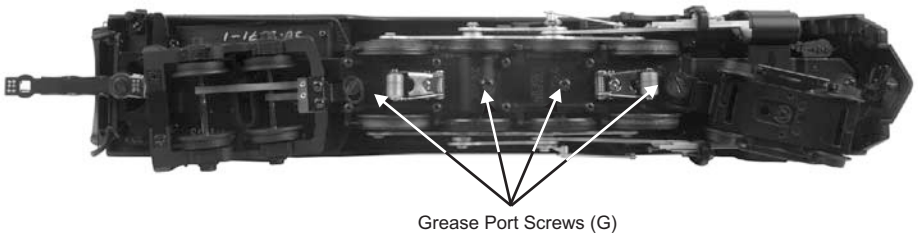
Figure 10: Grease Points
