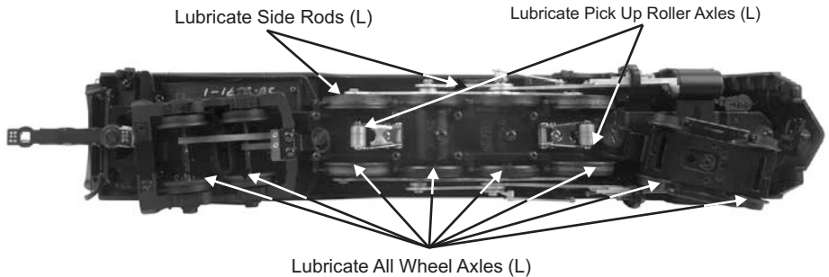
Fig. 1: Lubricating the Locomotive
