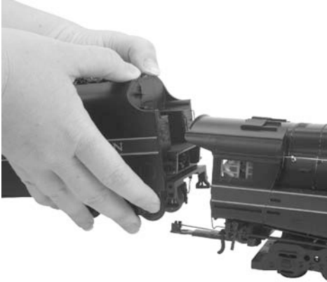
Figure 5: Connecting Locomotive to Tender
