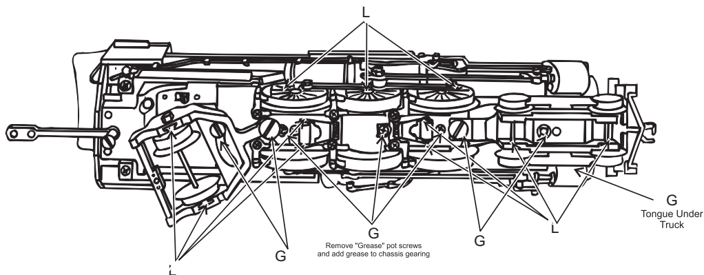
Figure 9: Lubricating The Locomotive Chassis
