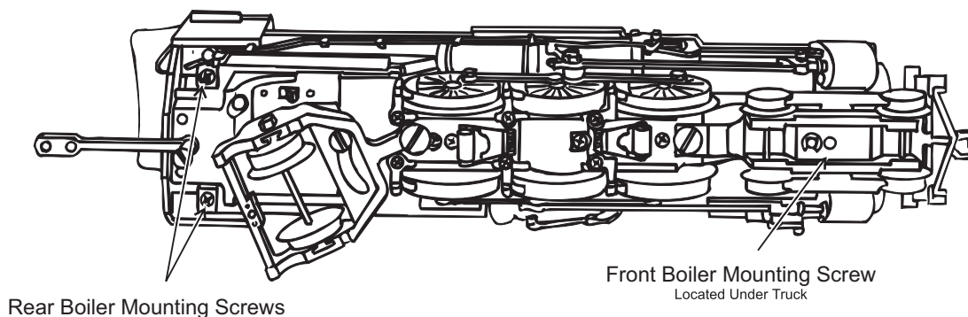
Figure 11: Removing The Boiler From The Chassis
