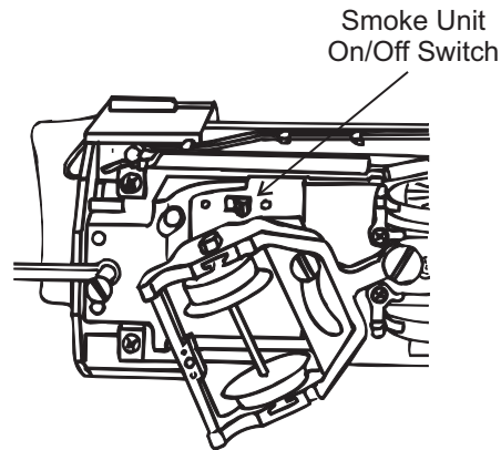
Figure 2: Smoke Unit On/Off Switch
