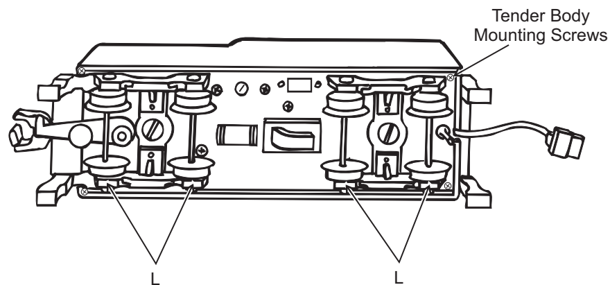
Figure 10: Lubricate The Tender Chassis Trucks Where The Axle Enters The Side Frame
