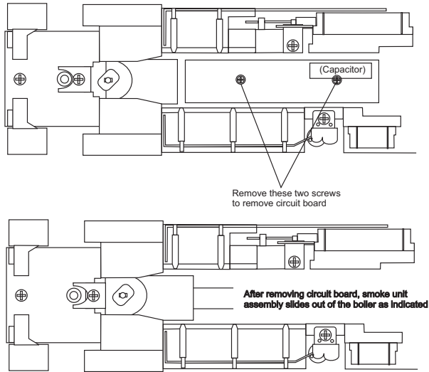
Figure 5: Inspecting the smoke wick
