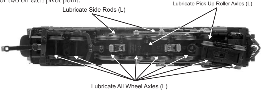
Fig. 9: Lubricating the Locomotive
