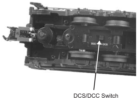
Figure 7: Changing from DCS to DCC Mode
