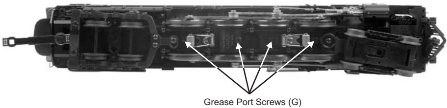
Figure 10: Grease Points
