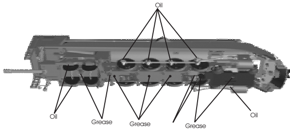
Figure 8: Lubricating The Locomotive Chassis
