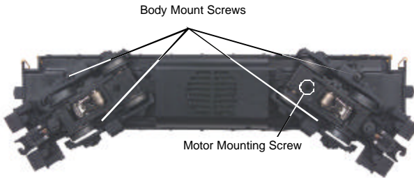
Figure 5: Body Removal Screw Locations
