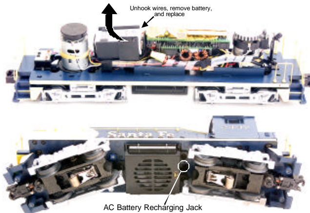
Figure 6. Replacing the Battery. Location of the Battery Re-charging Jack.
