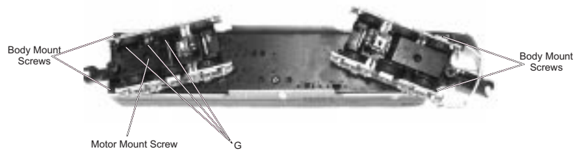
Figure 7: Lubricate The Tender Chassis Trucks
