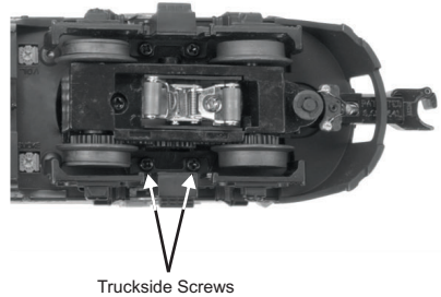
Figure 6: Truckside Screws
