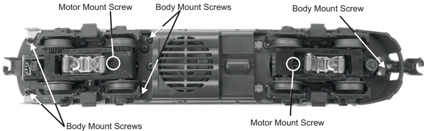
Figure 4: Motor Mount and Body Mount Screws
