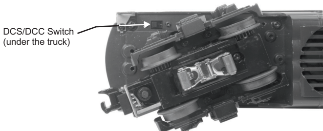
Figure 1: Changing from DCS to DCC Mode
