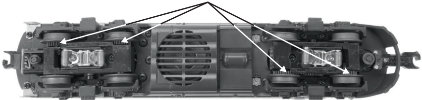
Figure 5: Greasing The Idler Gears
