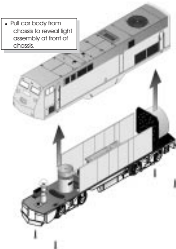
Figure 13: Lifting the body away from the chassis.
