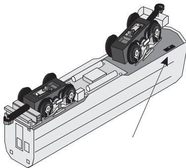
Figure 11: DCRU® Electronic Reverse Unit Lock-out Switch location.
