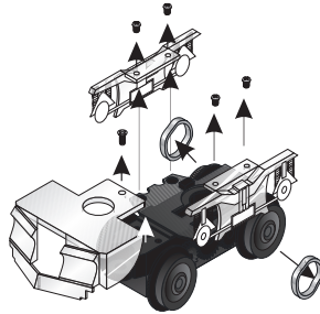
Figure 20: Removing locomotive trucksides for traction tire replacement.
