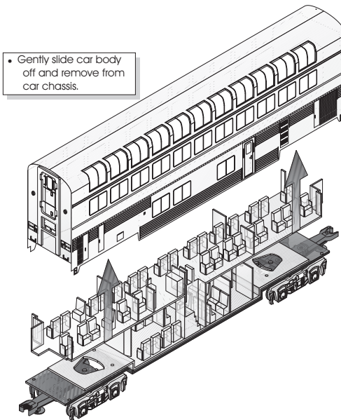
Figure 16: Removing the Superliner passenger car body from its chassis.
