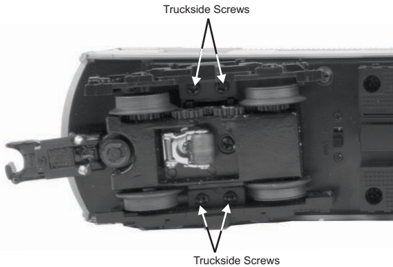
Figure 6: Truckside Screws
