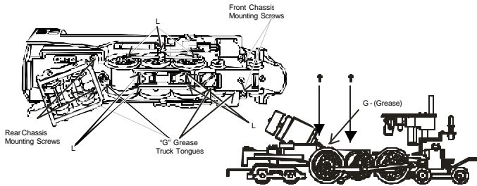
Figure 8: Lubricating The Locomotive Chassis
