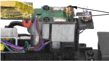
Remove Smoke Inspection Screws to Check Wick
