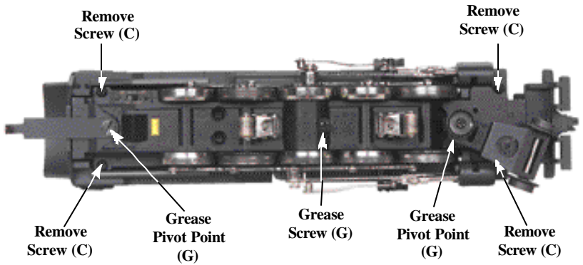
Figure 2 - Greasing (G) and Removing the Chassis (C) from Engine
