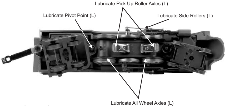
Figure 7: Lubricating the Locomotive
