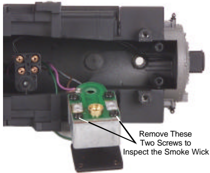
Figure 8. Inspecting the Smoke Unit's Wick
