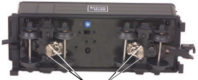
Lubricate Pick Up Rollers (L)
