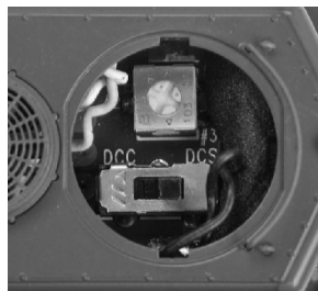
DCC-DCS Switch
